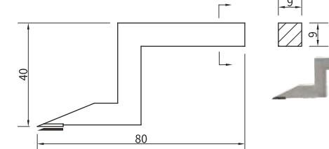
3110-4120 For:3110-6120-A Range:0-600/0-24"
