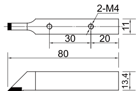
3001-4125 For:3001-0125,Range:0-1000/0-40"
