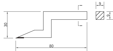
3110-4105 For:3110-6105-A Range:0-300/0-12"
