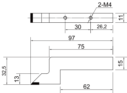
3001-4120 For:3001-0120,Range:0-600/0-24"
